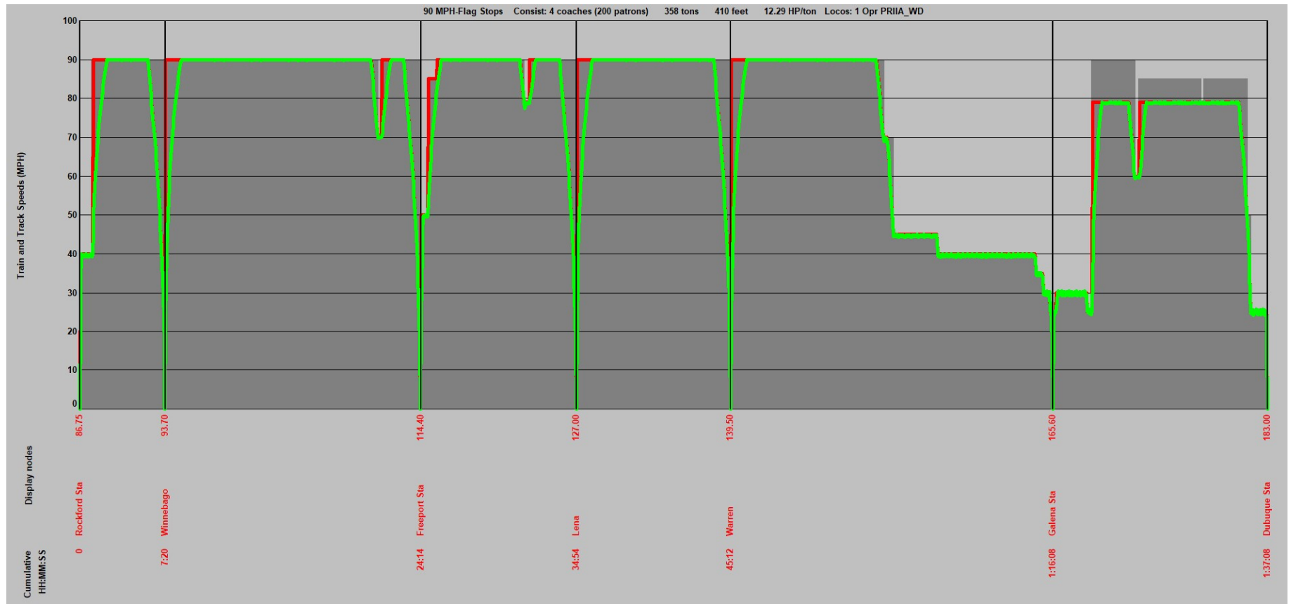
Pure Run Time Train Performance Calculator Output Chart – Primary and select secondary station stops at 90 MPH maximum speeds on CN
